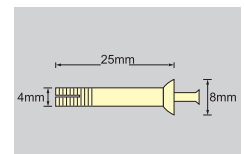
Anchor pin / dimensions
