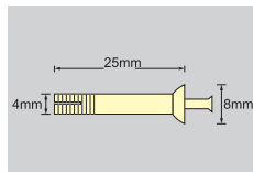
Anchor pin / dimension
